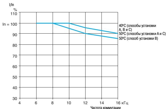
ATV 21HD30M3X
