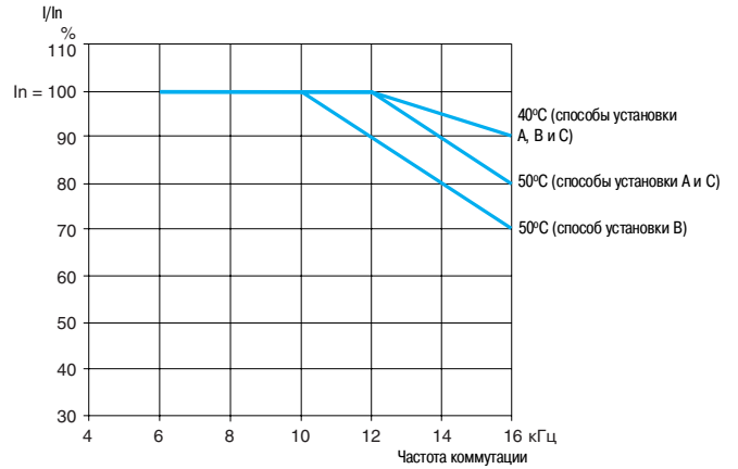
ATV 21HU22N4
