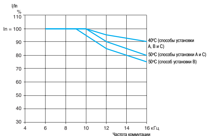
ATV 21HD22M3X
